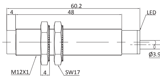
Fig. 4 Inductive sensor with cable (non-flush)
