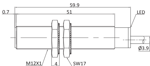
Fig. 3 Inductive sensor with cable (flush)
