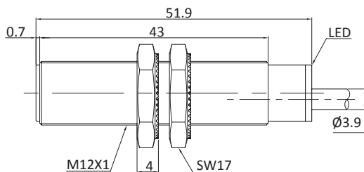
Fig. 1 Inductive sensor with cable (flush)
